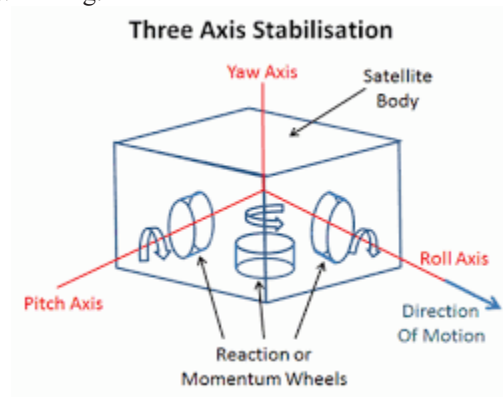
Figure 2. The Layout of attitude control using RWs
