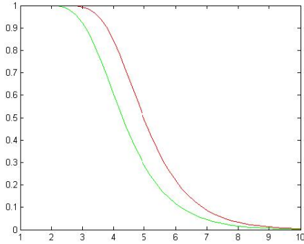
Figure 1. The reliability function for n=50,100
