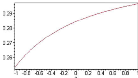
Figure 3. Graph of M_{1,1}(t) , \alpha = 0.5 , n = 4
